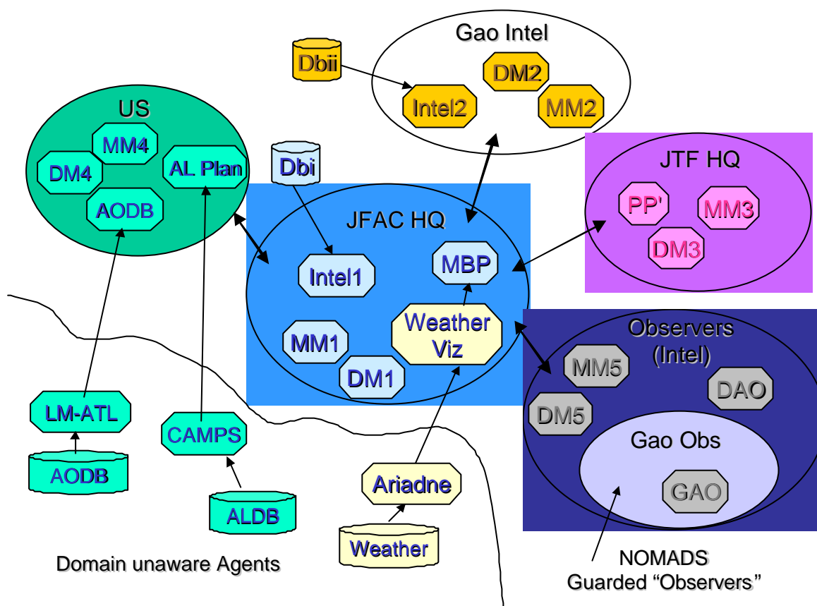
Figure 4 - Software Agent Domain Mappings
