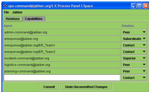
Figure 3: The I-Space Tool. The agents’ relations to each other govern the nature of interactions between them.
