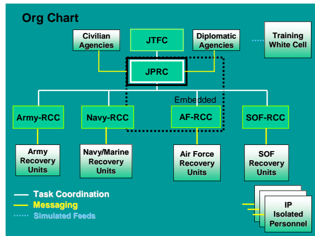
Figure 5: Organization of Agents in the Scenario
